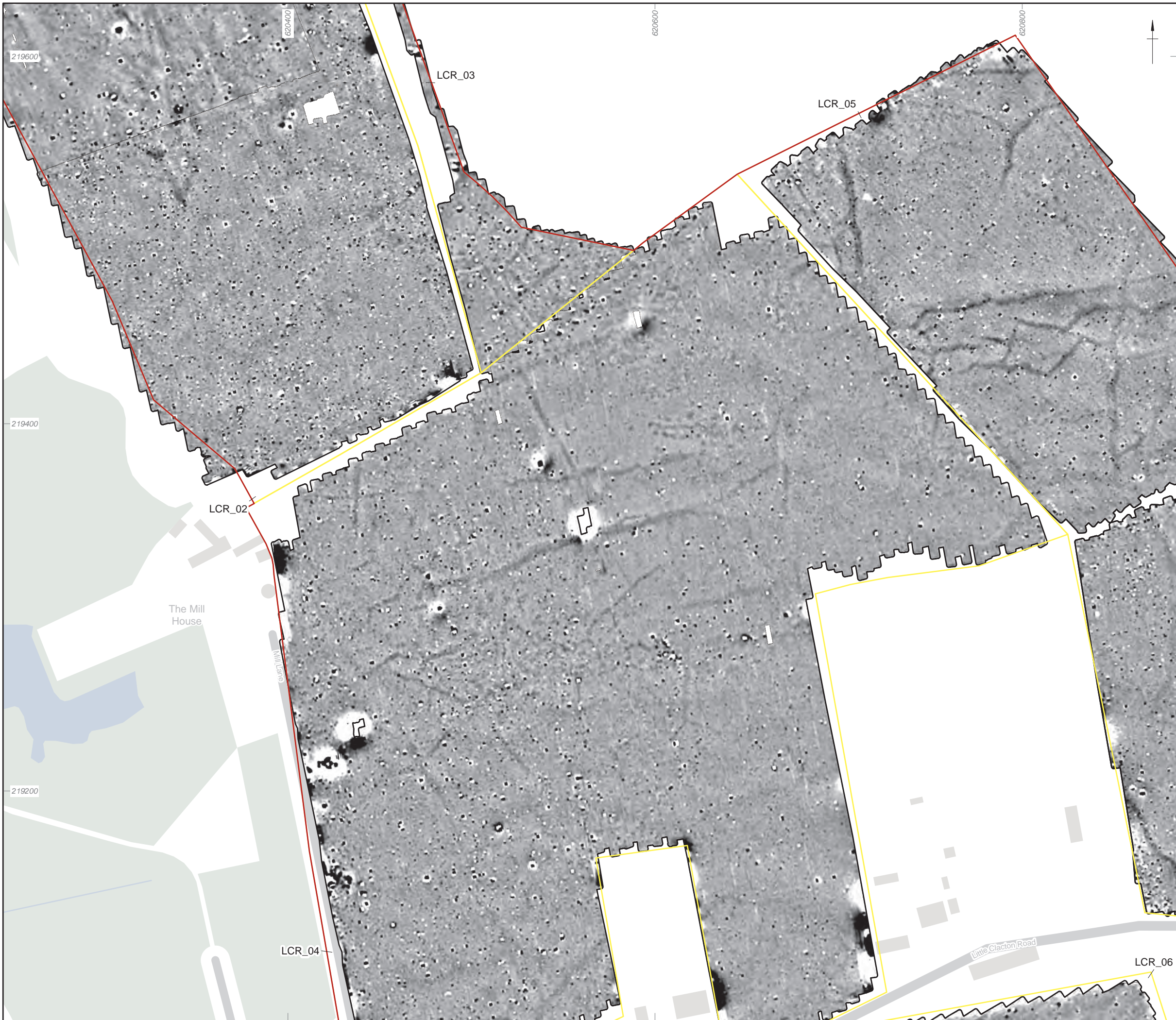
Figure 110: Detailed gradiometer survey results: greyscale plot (LCR_2, LCR_3, LCR_4, LCR_5)
