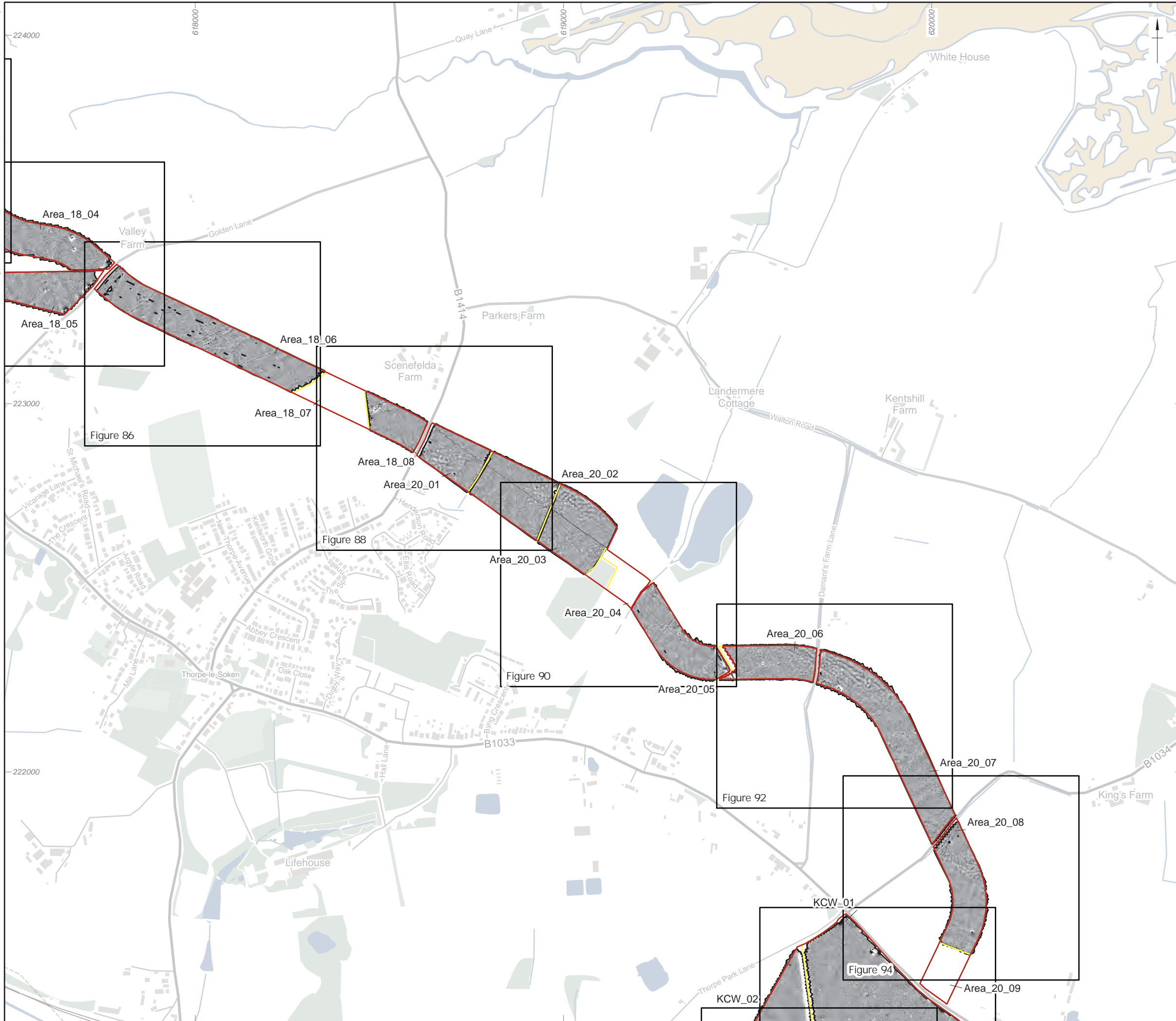
Figure 10: Detailed gradiometer survey results: overview greyscale plot (Area 18, Area 20)
