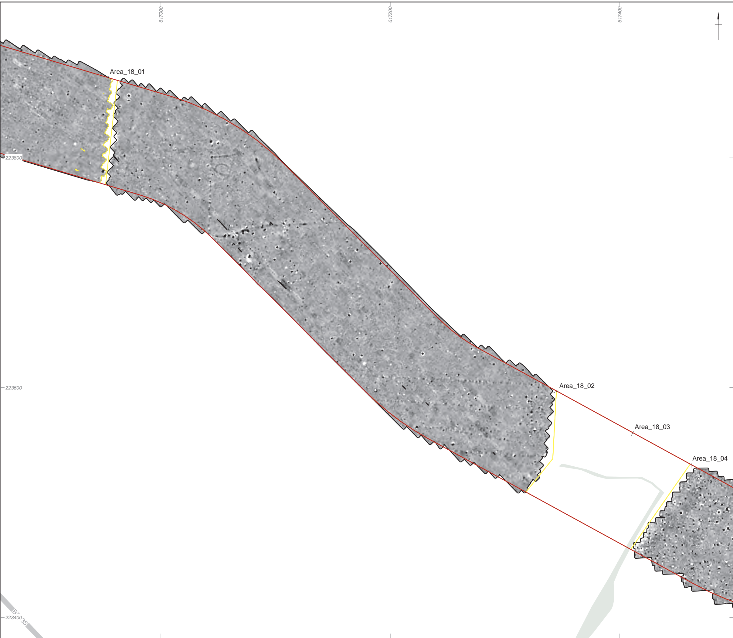
Figure 82: Detailed gradiometer survey results: greyscale plot (Area_18_02, Area_18_03)
