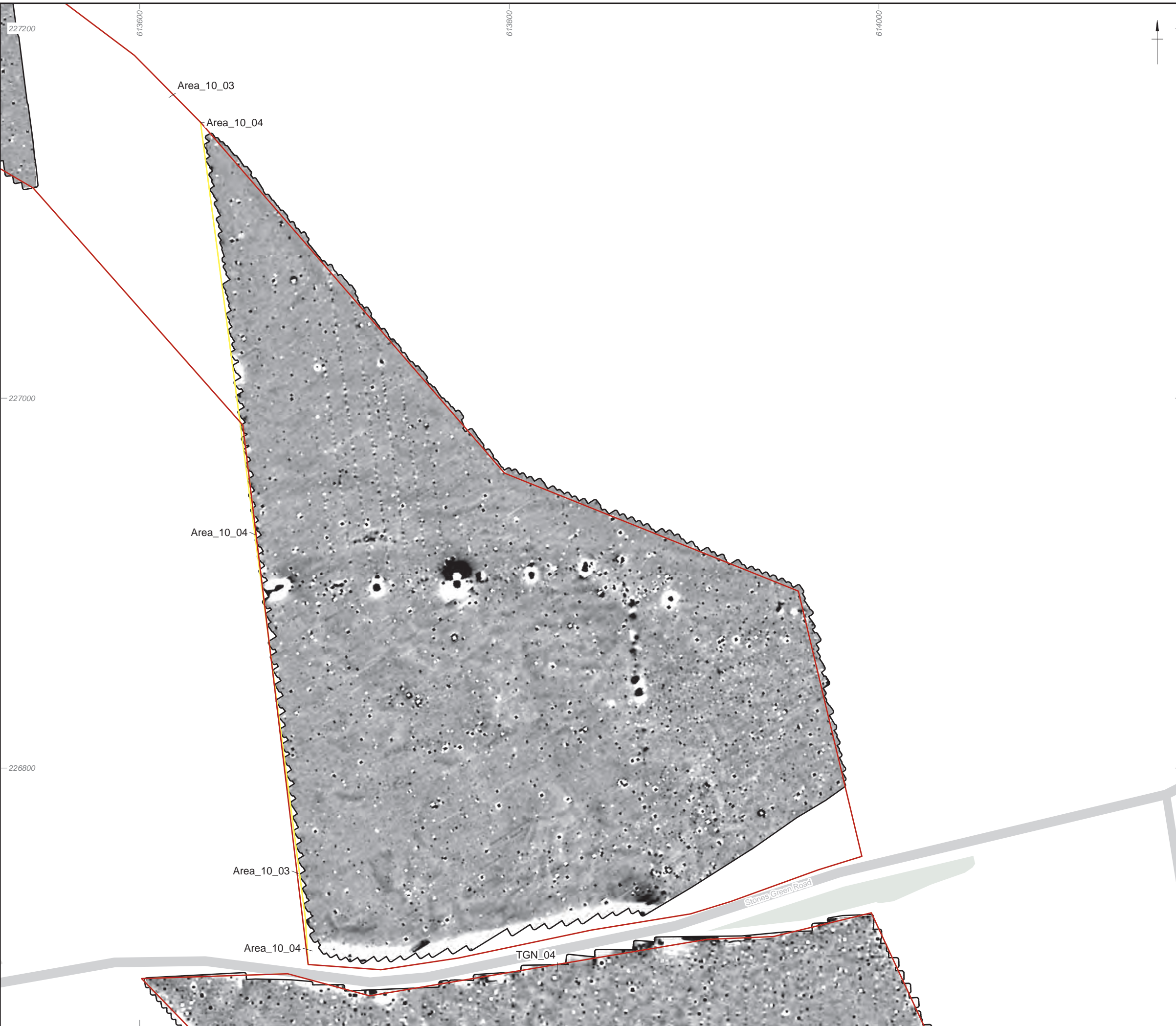
Figure 58: Detailed gradiometer survey results: greyscale plot (Area_10_04)
