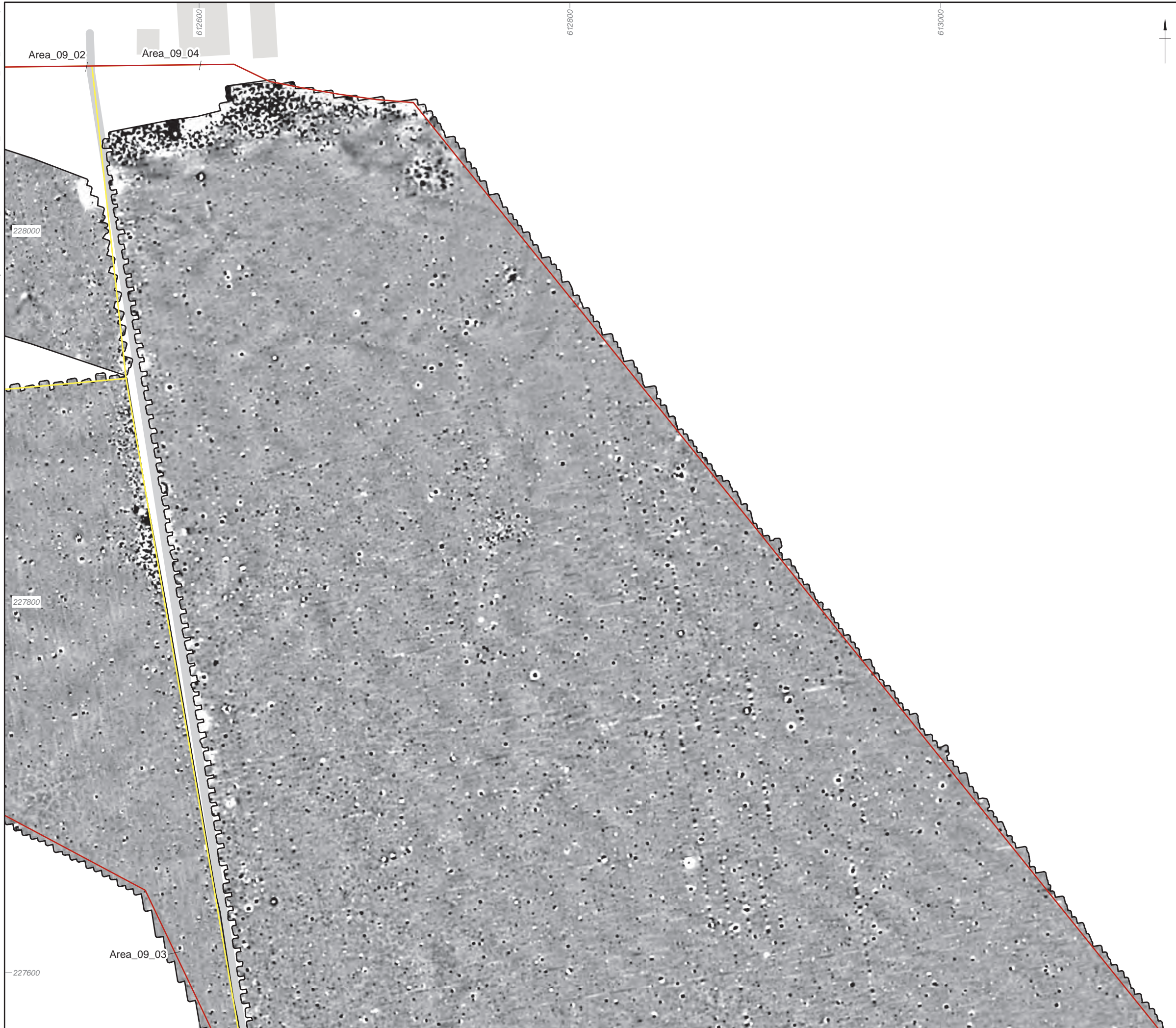
Figure 50: Detailed gradiometer survey results: greyscale plot (Area_09_04)
