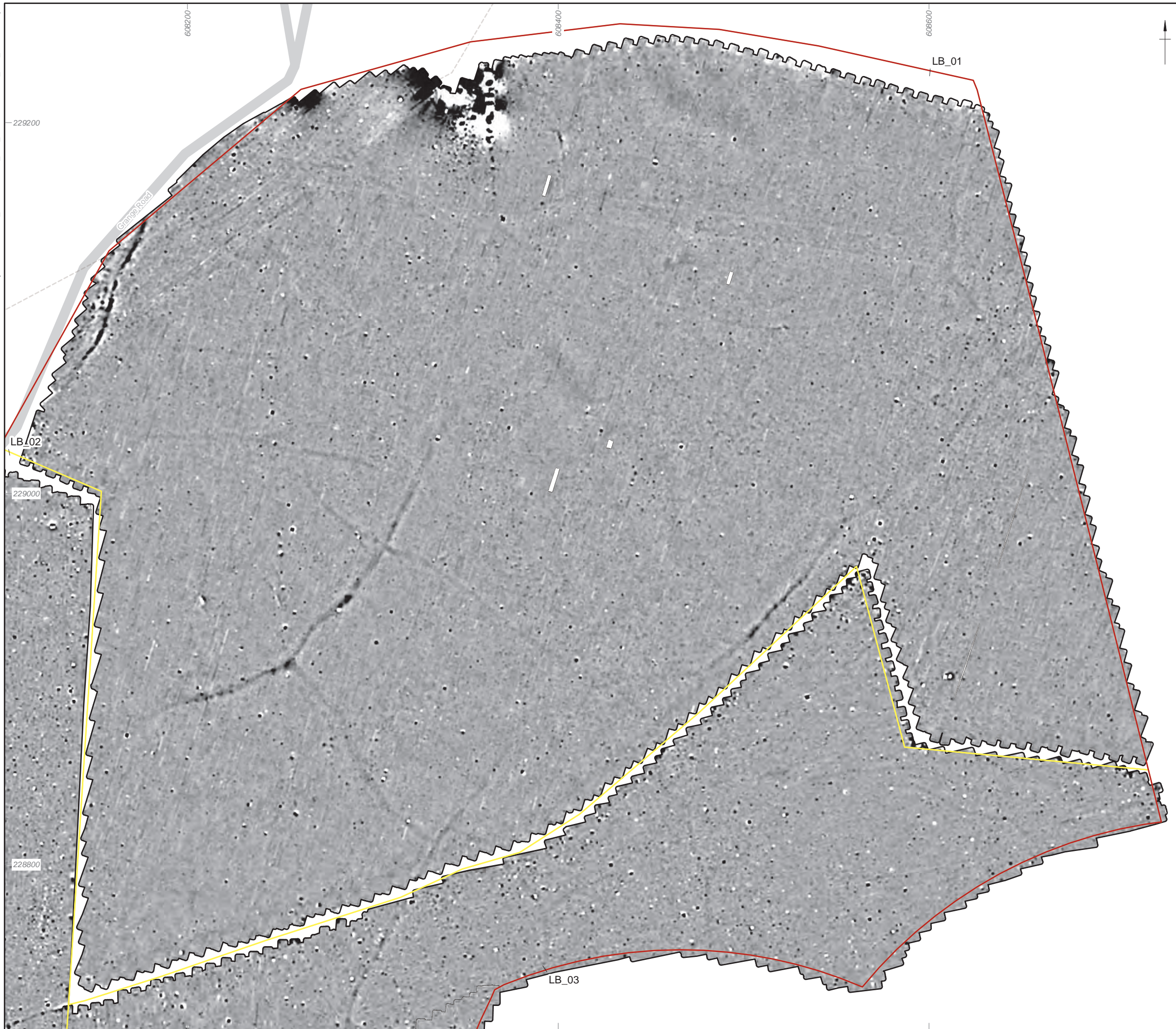
Figure 16: Detailed gradiometer survey results: greyscale plot (LB_1, LB_3)
