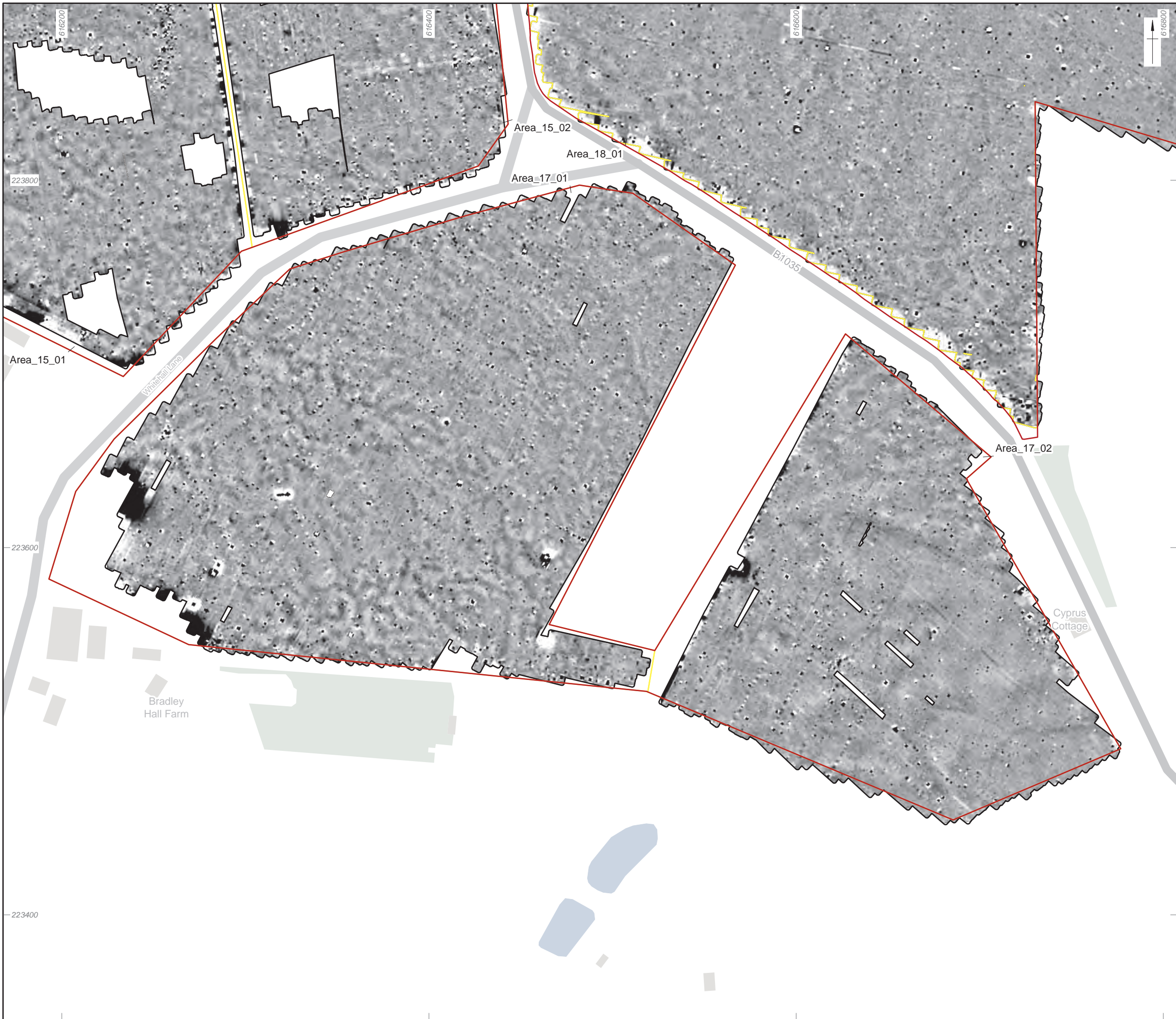
Figure 78: Detailed gradiometer survey results: greyscale plot (Area_17_01, Area_17_02)
