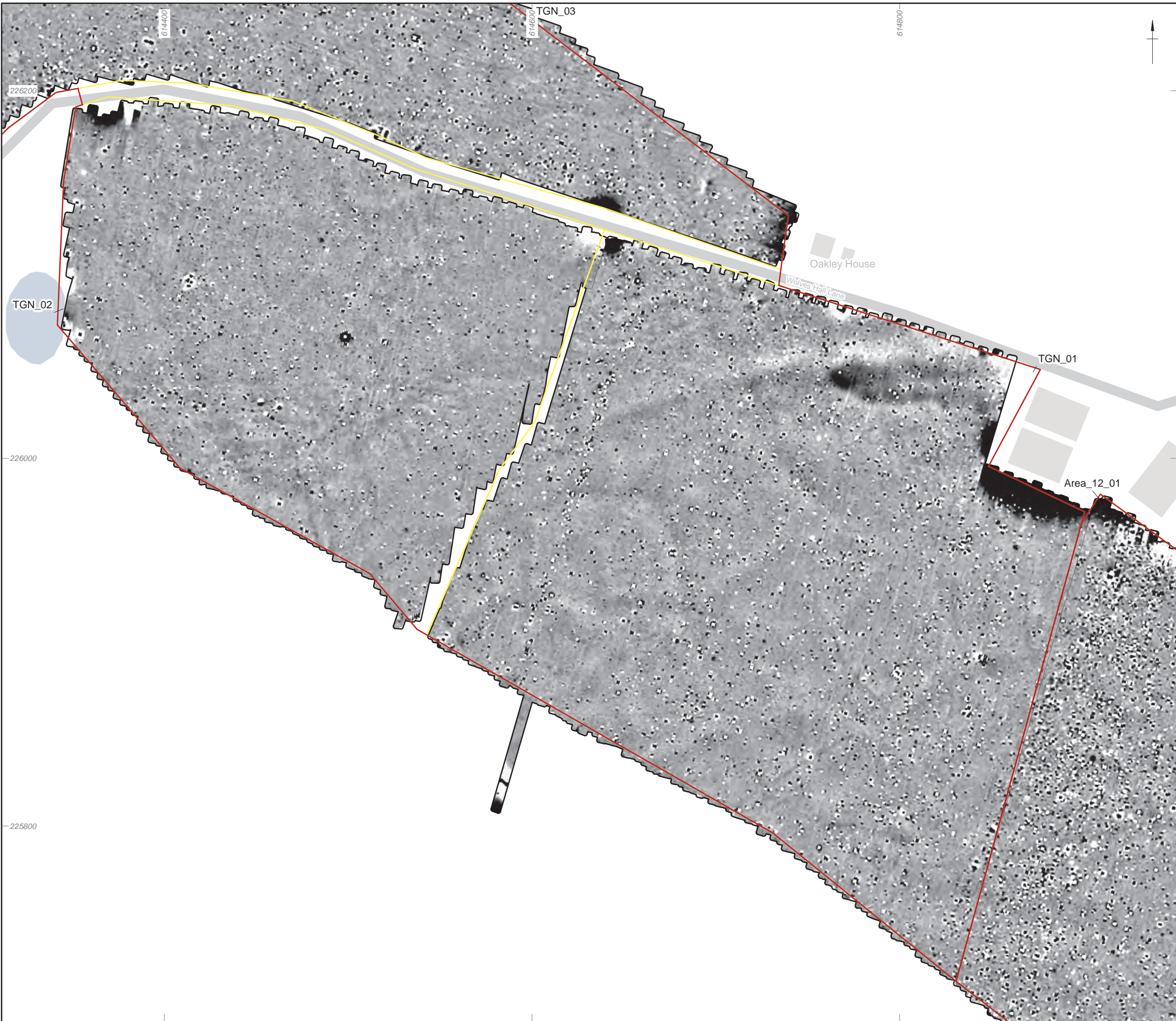
Figure 64: Detailed gradiometer survey results: greyscale plot (TGN_01, TGN_02)
