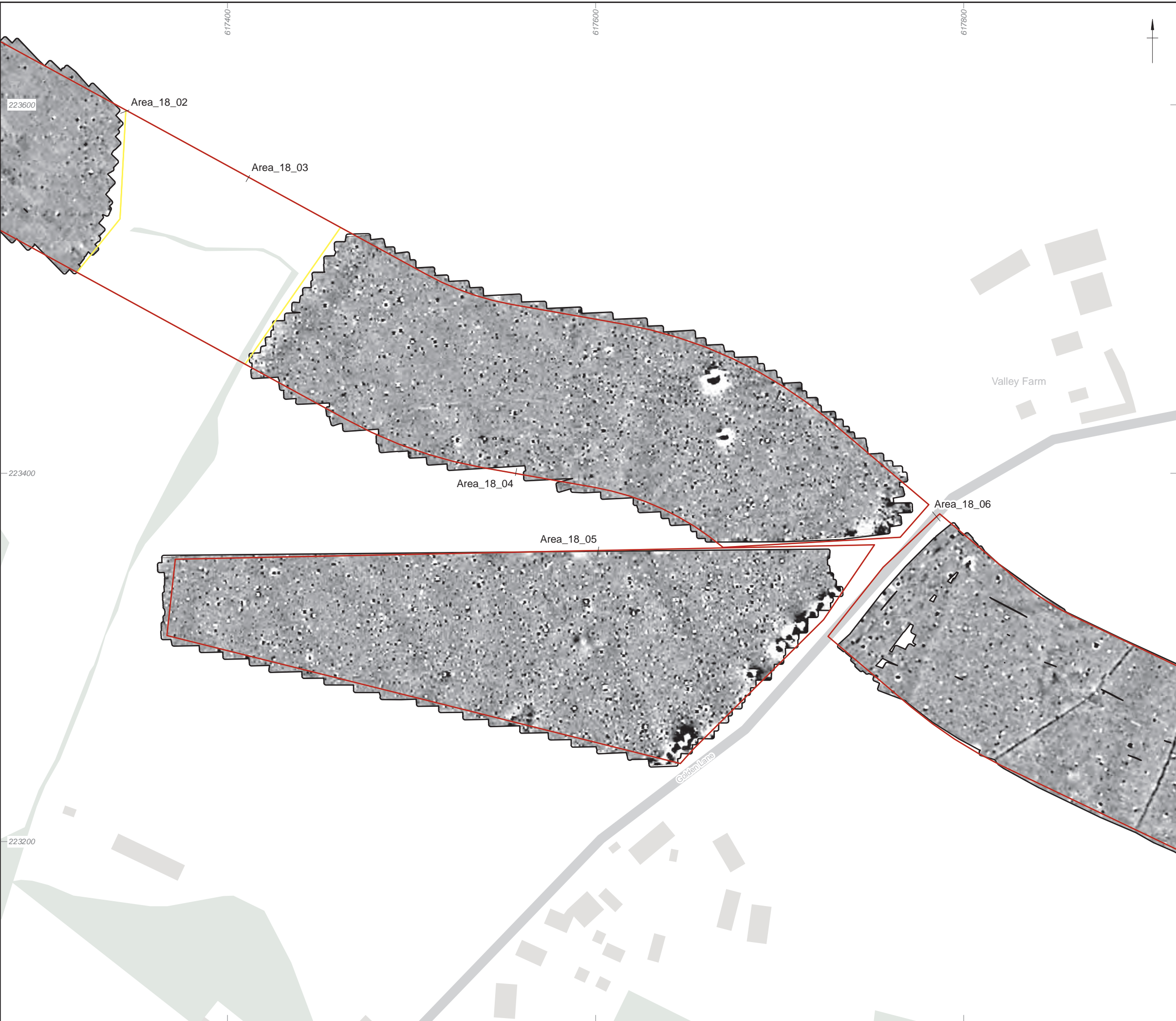
Figure 84: Detailed gradiometer survey results: greyscale plot (Area_18_04, Area_18_05)
