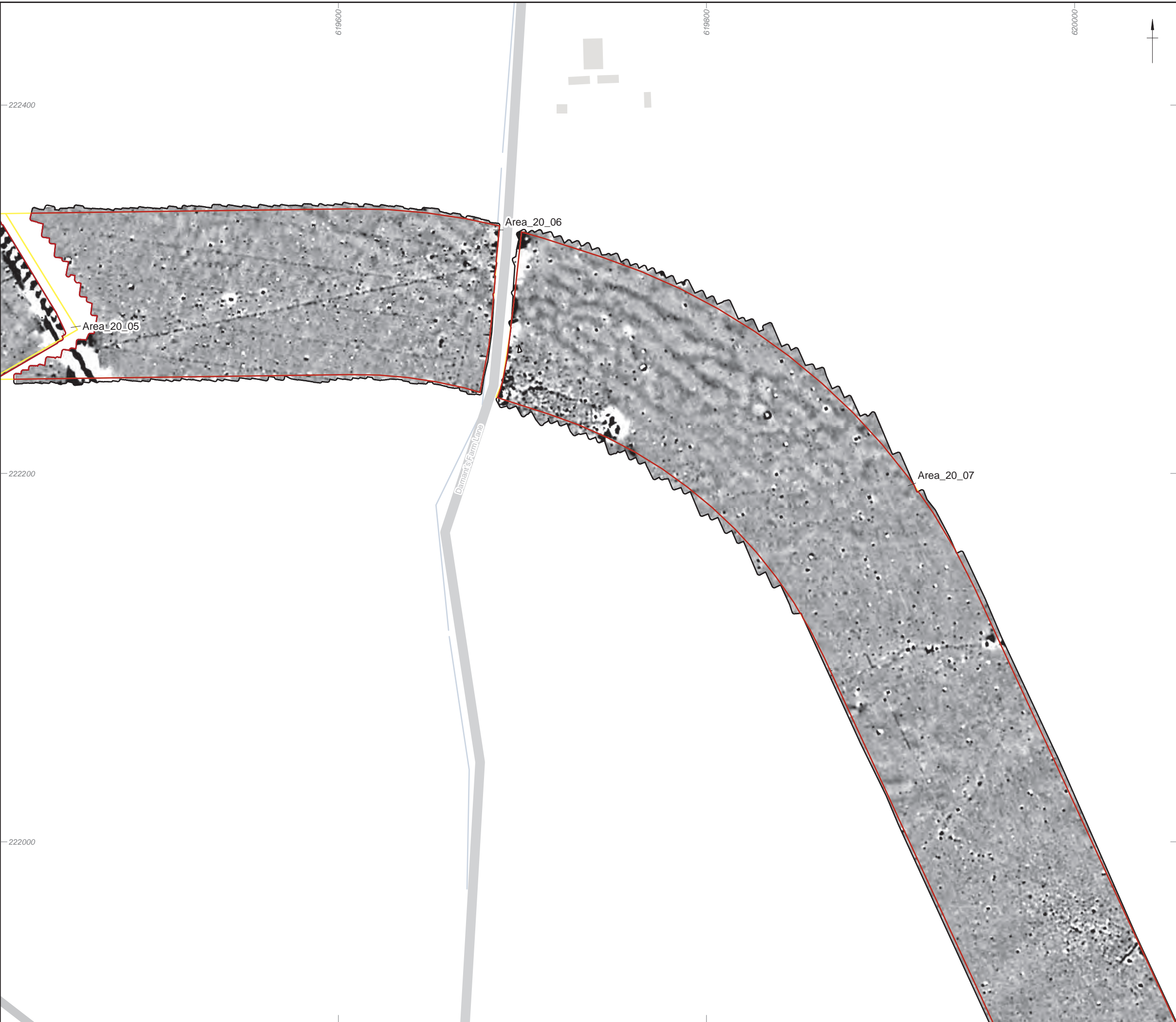
Figure 92: Detailed gradiometer survey results: greyscale plot (Area_20_06)
