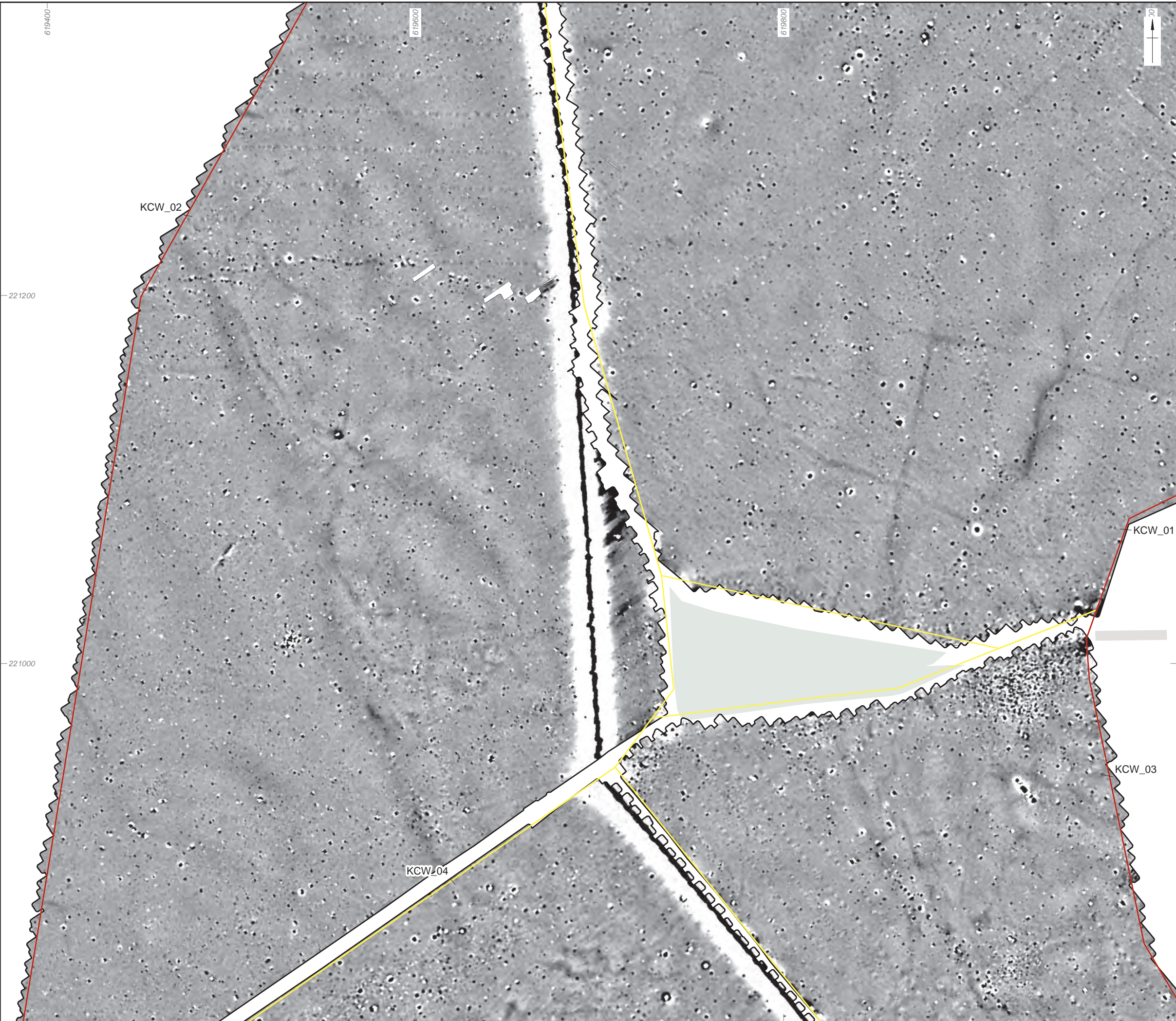
Figure 98: Detailed gradiometer survey results: greyscale plot (KCW_01, KCW_02, KCW_03, KCW_04)
