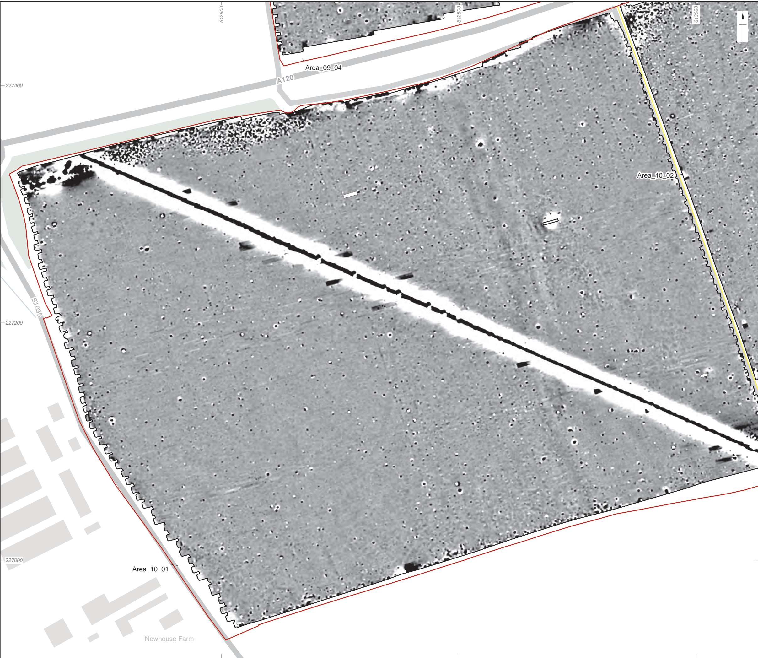
Figure 54: Detailed gradiometer survey results: greyscale plot (Area_10_01)
