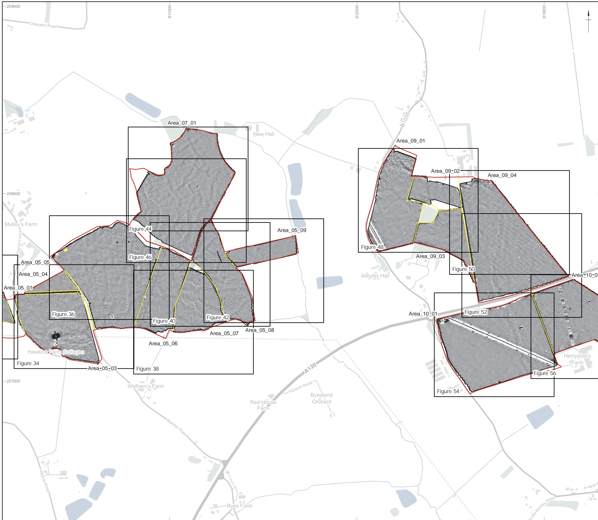
Figure 4: Detailed gradiometer survey results: overview greyscale plot (Area 5, Area 7, Area 9, Area 10)
