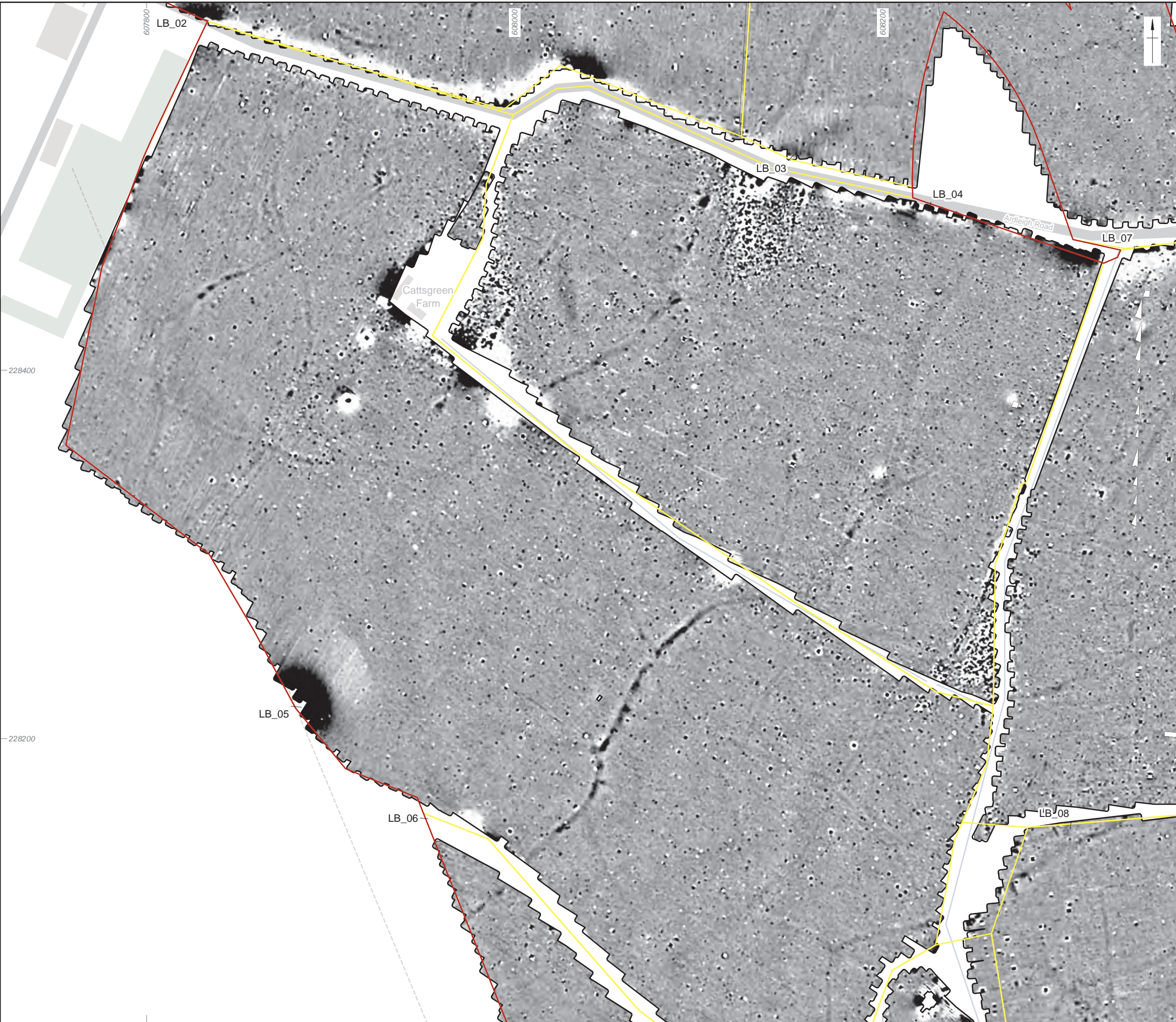
Figure 22: Detailed gradiometer survey results: greyscale plot (LB_4, LB_5, LB_7, LB_8)
