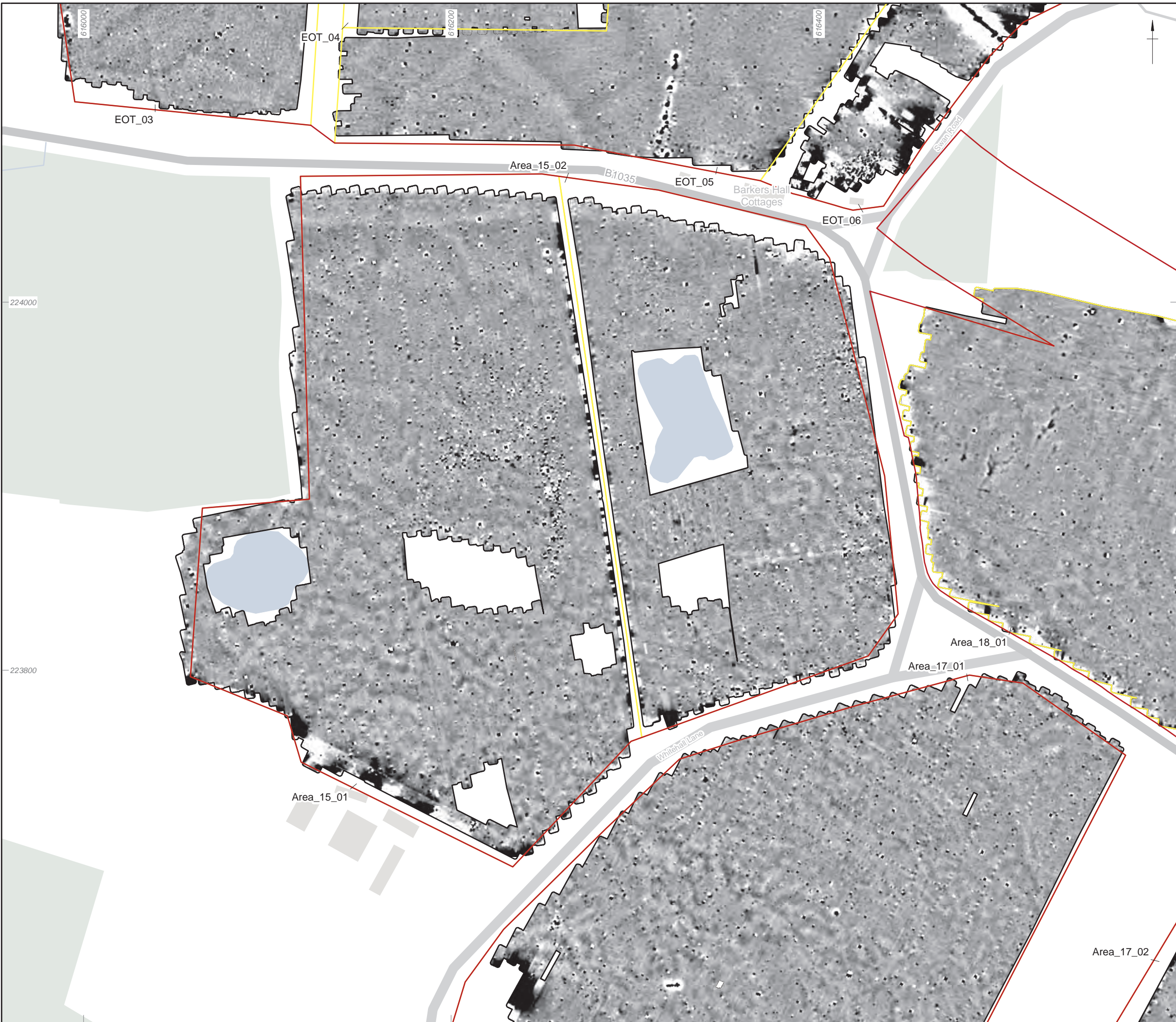
Figure 76: Detailed gradiometer survey results: greyscale plot (Area_15_01, Area_15_02)
