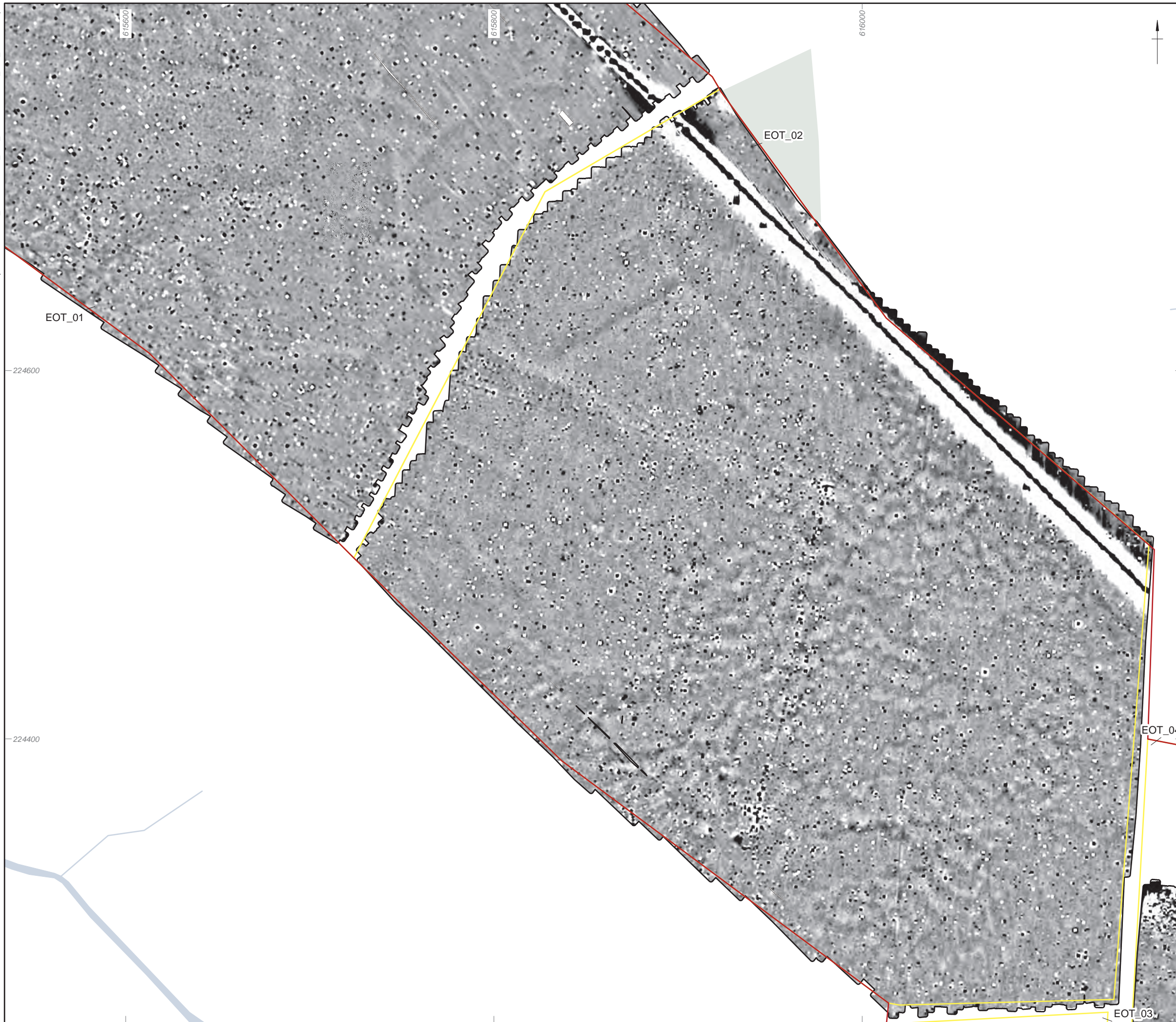
Figure 72: Detailed gradiometer survey results: greyscale plot (EOT_02)
