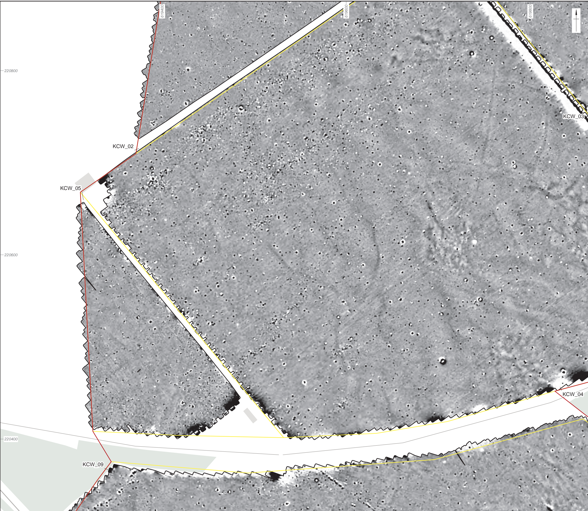
Figure 100: Detailed gradiometer survey results: greyscale plot (KCW_04, KCW_05)
