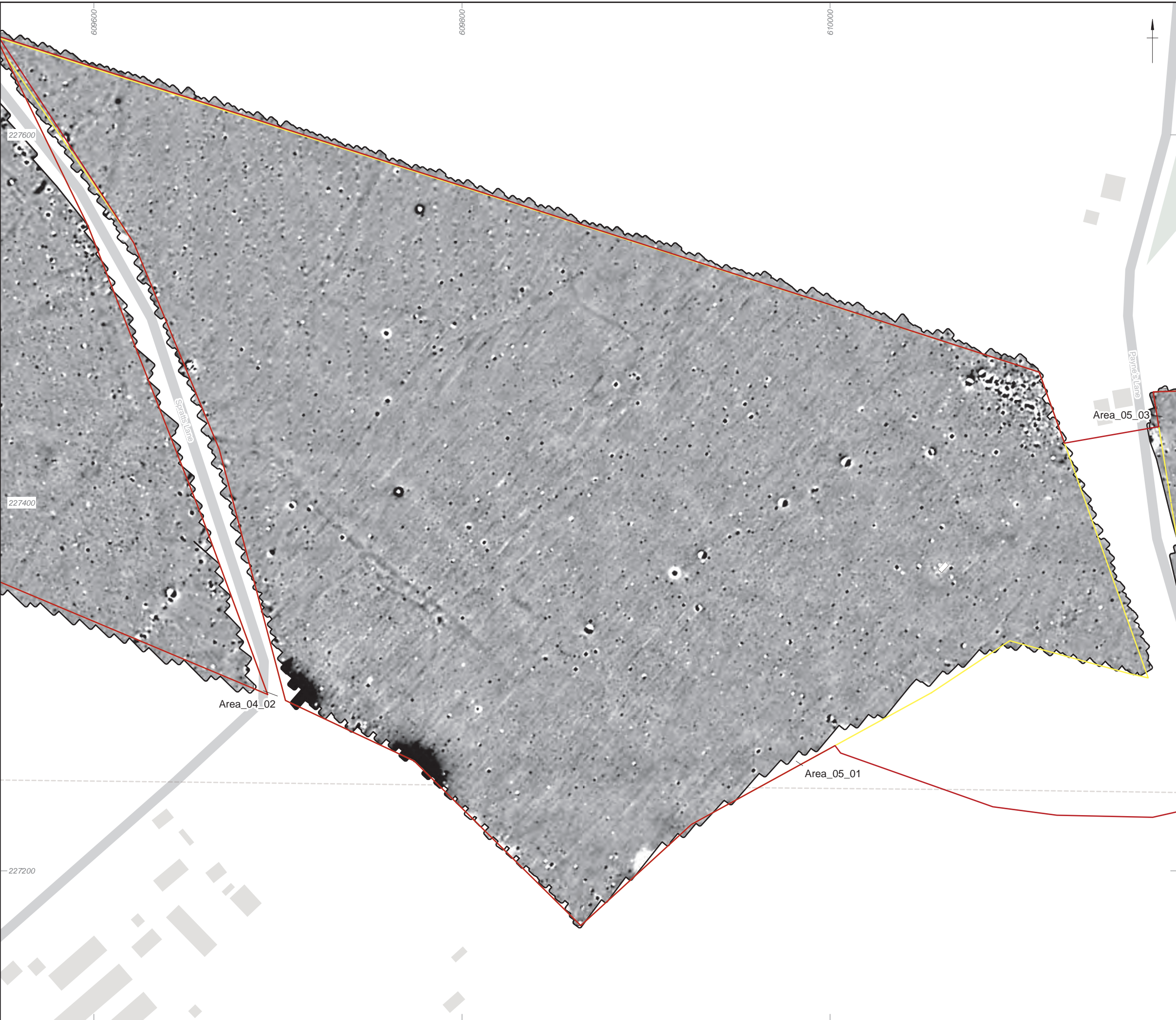
Figure 32: Detailed gradiometer survey results: greyscale plot (Area_04_02, Area_5_01)
