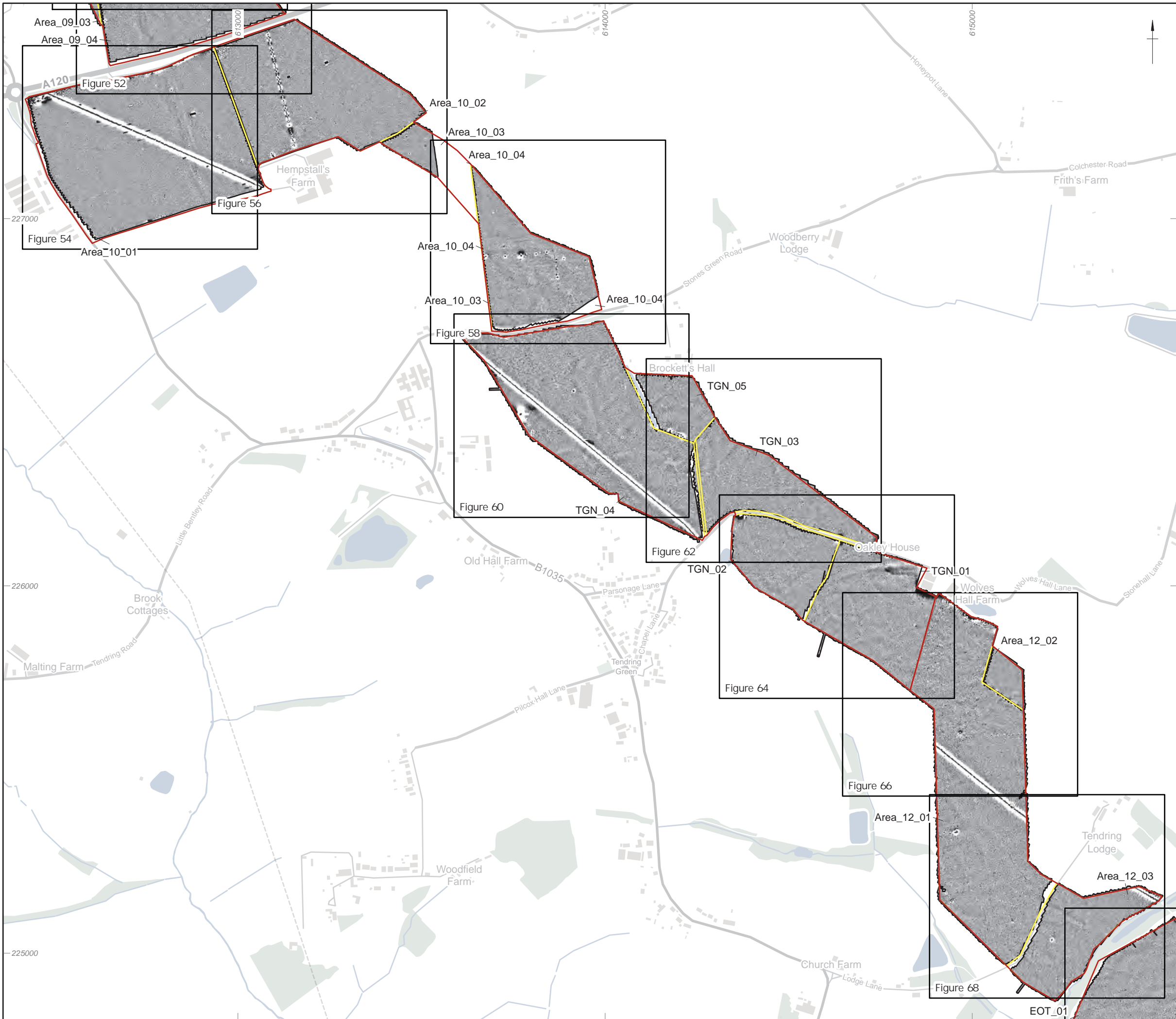
Figure 6: Detailed gradiometer survey results: overview greyscale plot (Area 10, Tending Green North, Area 12)
