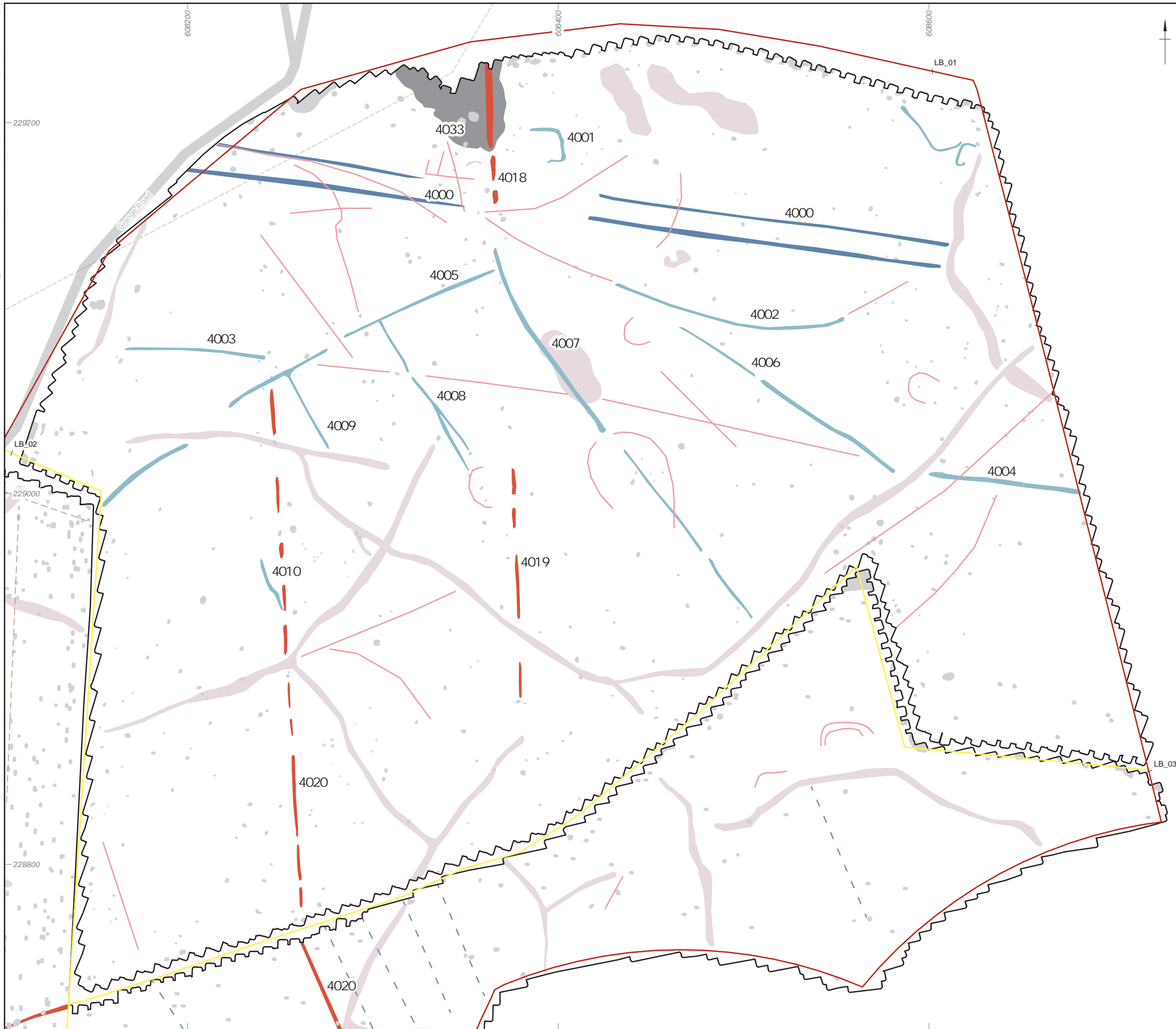
Figure 17: Detailed gradiometer survey results: interpretation(LB_1, LB_3)
