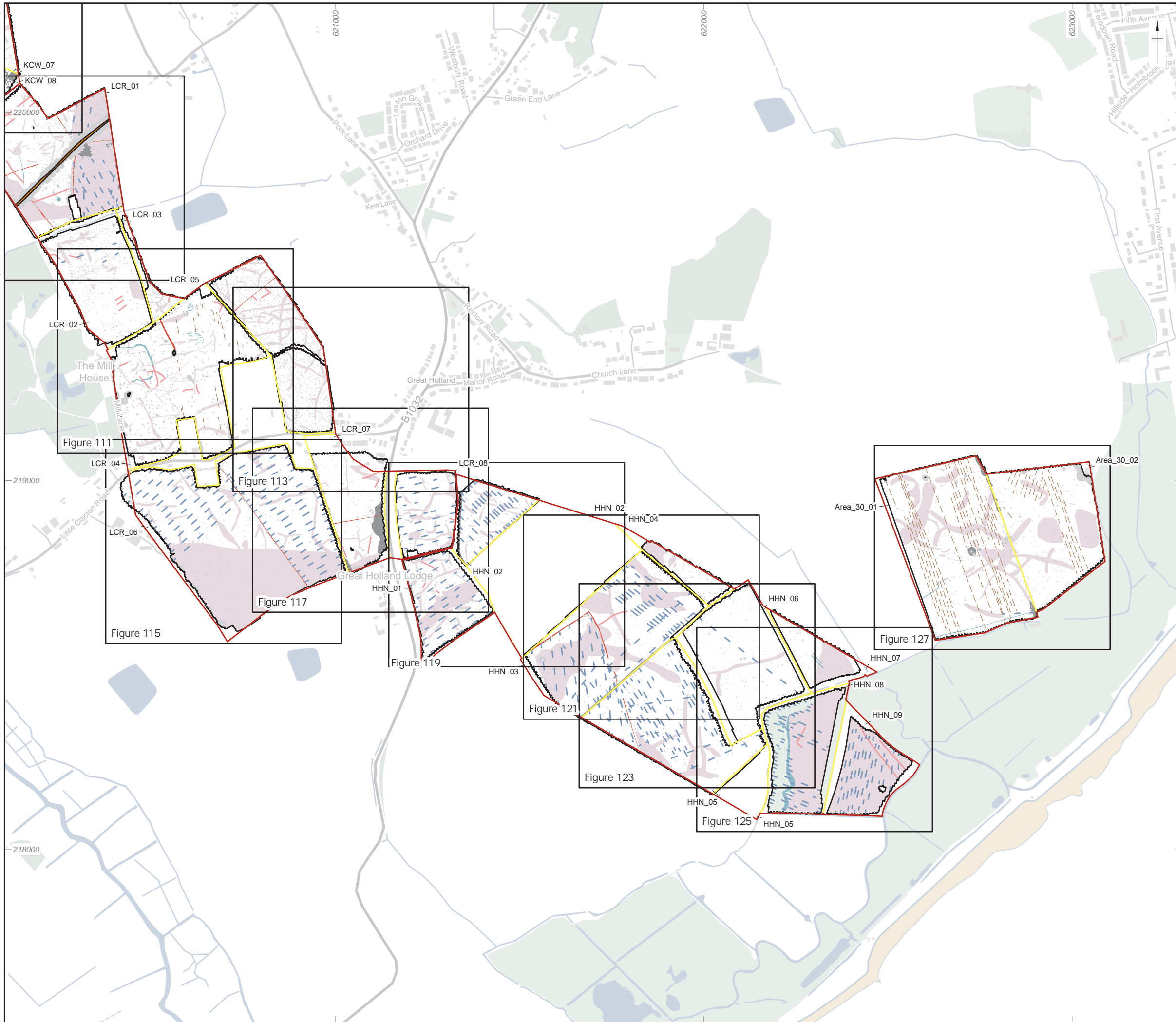
Figure 15: Detailed gradiometer survey results: overview interpretation (Little Clacton Road, Holadn Haven North, Area 30)
