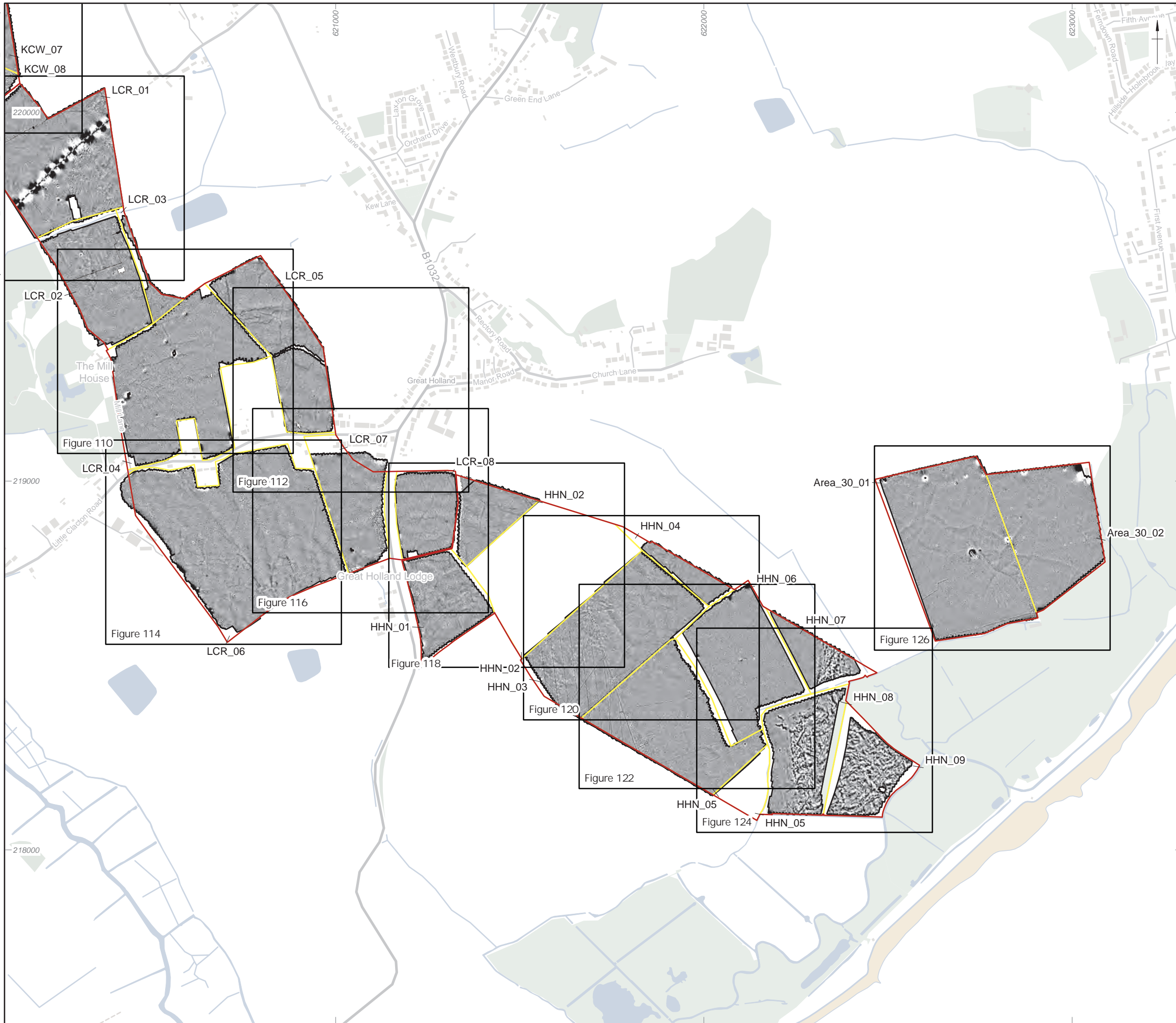
Figure 14: Detailed gradiometer survey results: overview greyscale plot (Little Clacton Road, Holadn Haven North, Area 30)
