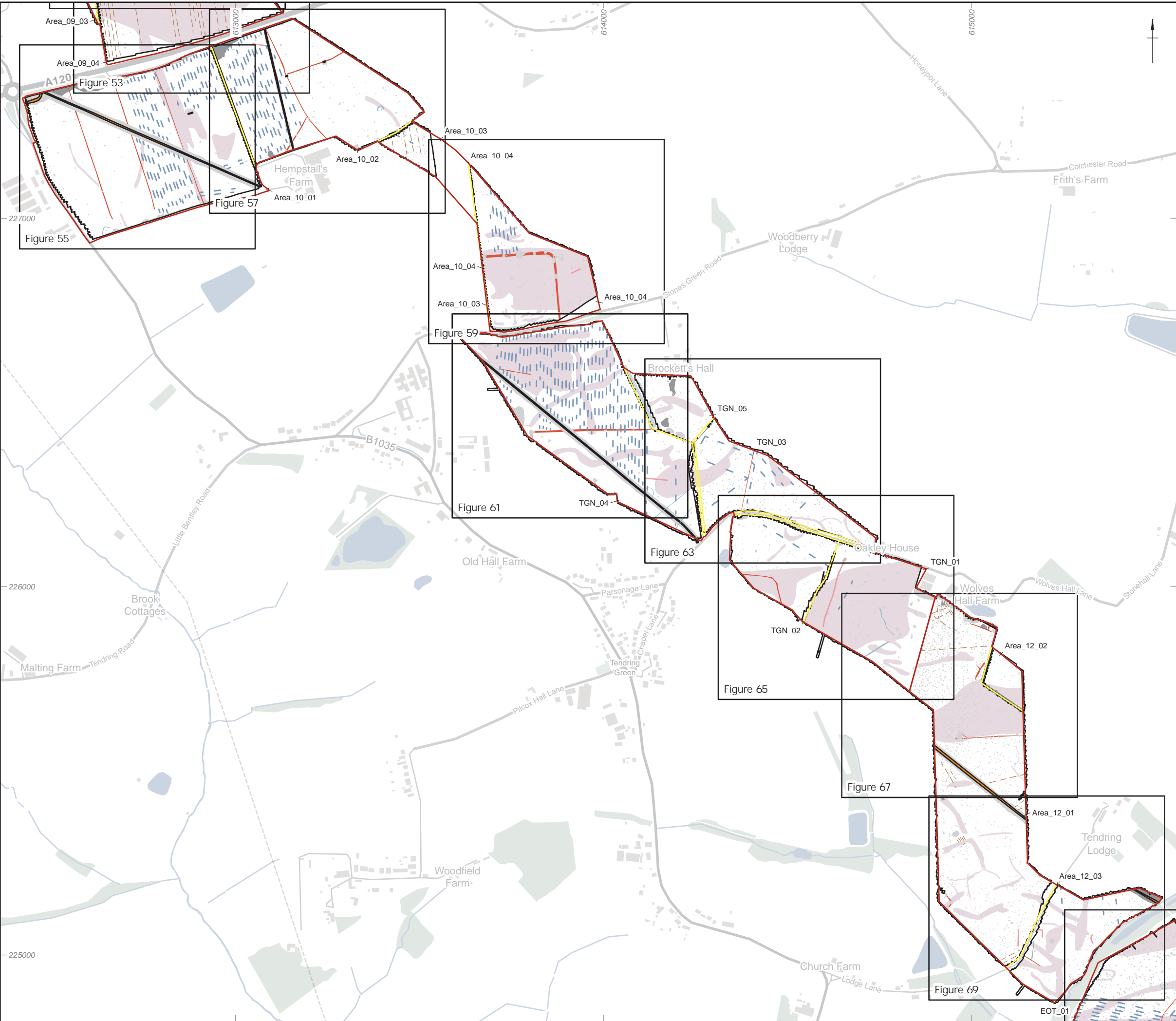
Figure 7: Detailed gradiometer survey results: overview interpretation (Area 10, Tending Green North, Area 12)
