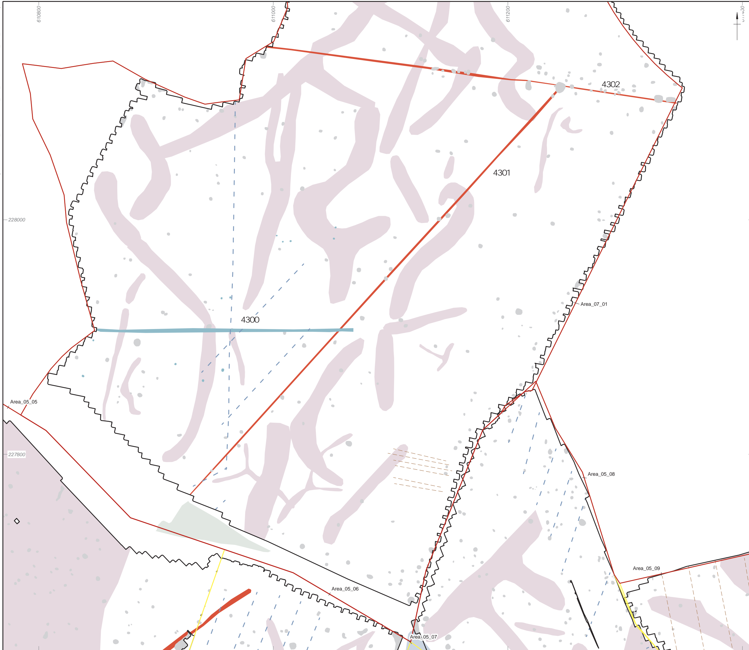
Figure 47: Detailed gradiometer survey results: interpretation(Area_7 (South))
