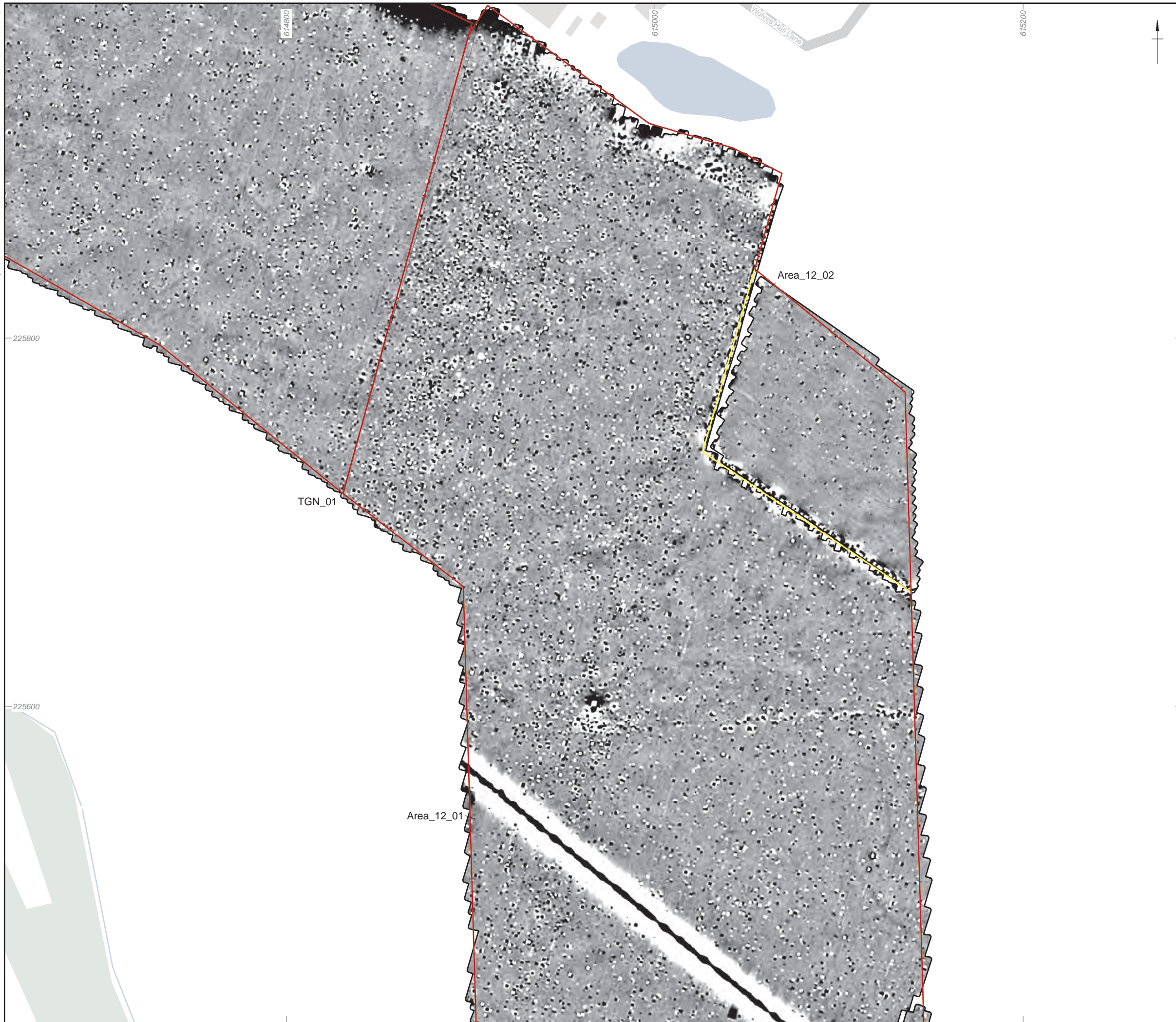
Figure 66: Detailed gradiometer survey results: greyscale plot (Area_12_01, Area_12_02)
