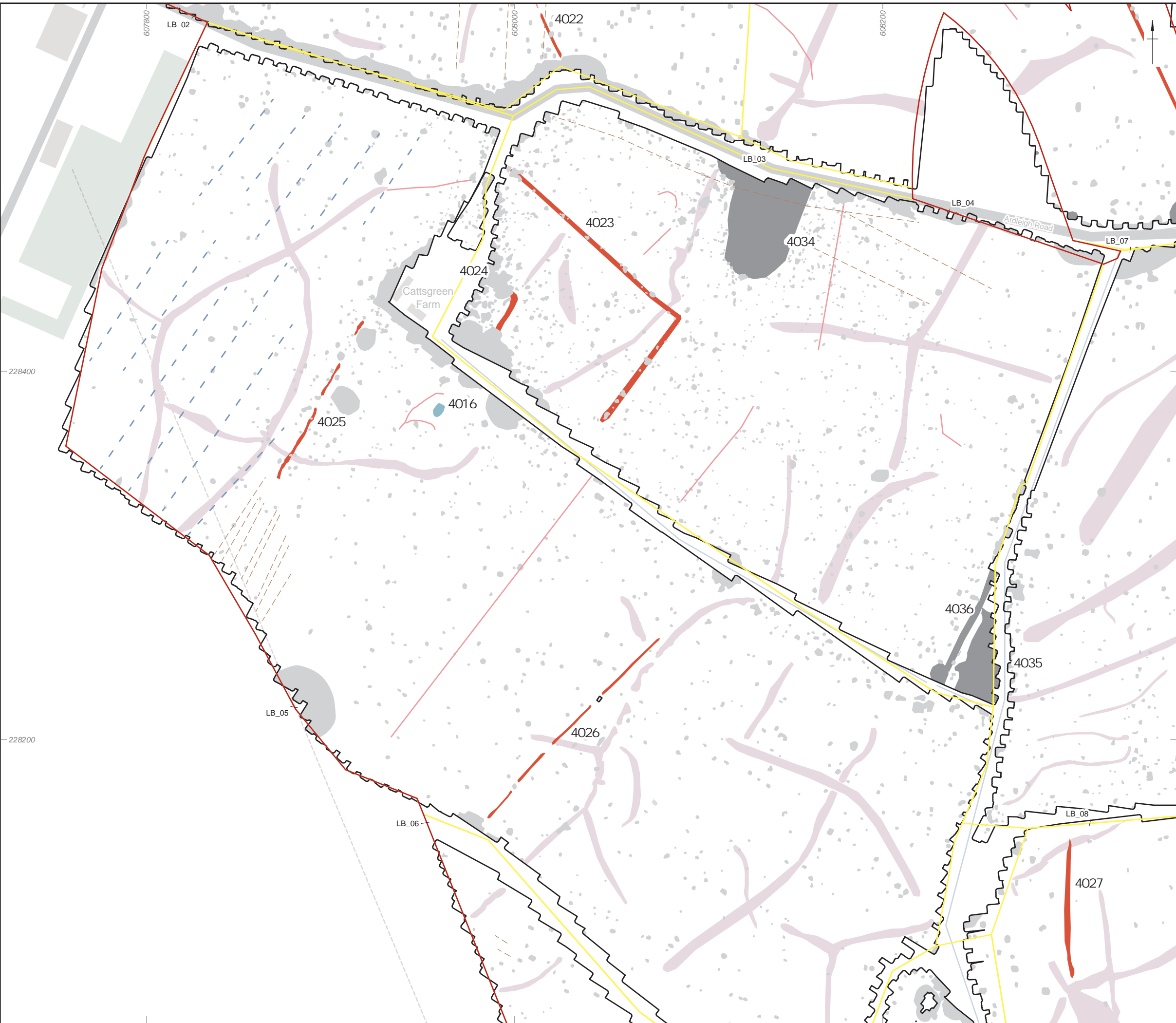
Figure 23: Detailed gradiometer survey results: interpretation(LB_4, LB_5, LB_7, LB_8)
