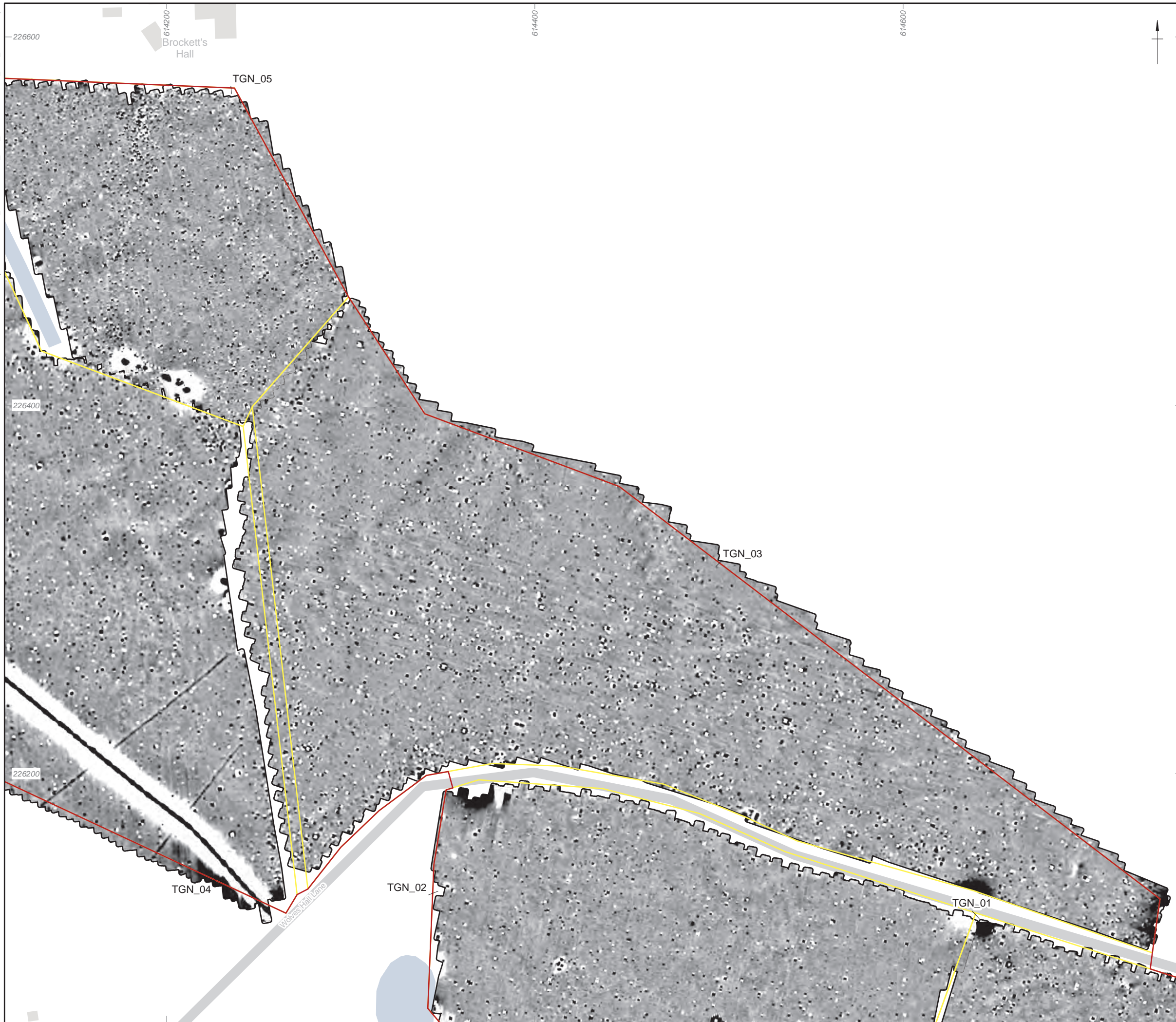
Figure 62: Detailed gradiometer survey results: greyscale plot (TGN_03, TGN_05)
